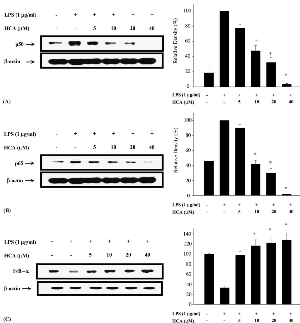
Fig. 5. Effect of HCA on LPS-induced NF- \kappa B activity and degradation of I \kappa B. The cells were treated with 1 \mu g/ml of LPS only or LPS plus different concentrations (5, 10, 20 and 40 \mu M) of HCA at 37 °C for 1 h. Equal amounts of total proteins (50 \mu g/lane) were subjected to 10% SDS-PAGE. Nuclear translocation of p50 (A) and p65 (B), and degradation of I \kappa B (C) were detected by Western blotting using specific antibodies. \beta -Actin protein was used here as an internal control. Quantification of band intensities from three independent experimental results was determined by a densitometry (Imaging System). Data was described as mean \pm S.E.M. from three experiments performed in triplicate for p50, p65, or I \kappa B/ \beta -actin. * P < 0.05 indicate statistically significant differences from the LPS-treated group.
